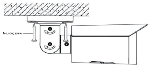
Figure 2-2 Fixed camera
