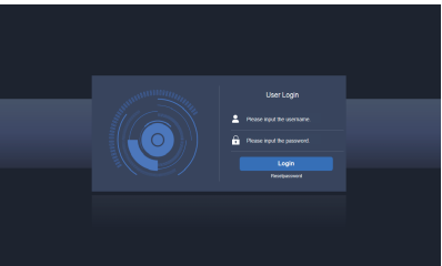
Figure 3- 2 Login
